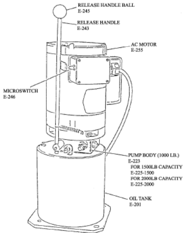
Figure 14: Standard AC Power Pack
