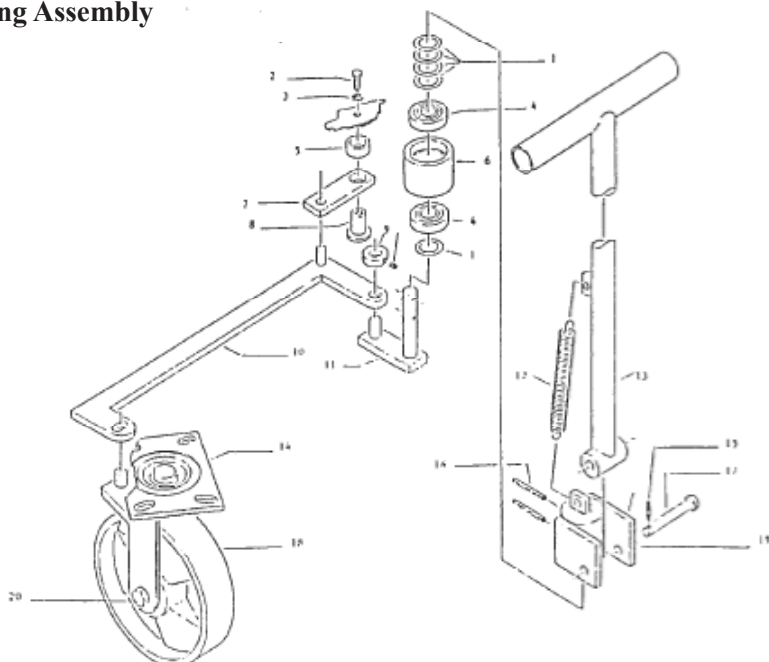
Figure 4: Steering Assembly
