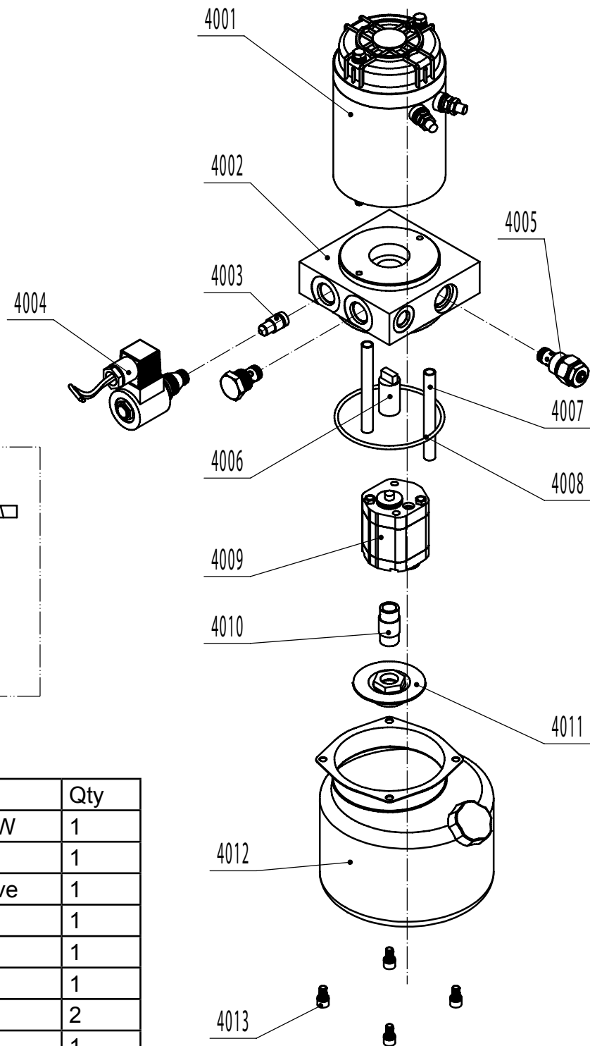
Figure 6. Power Unit
